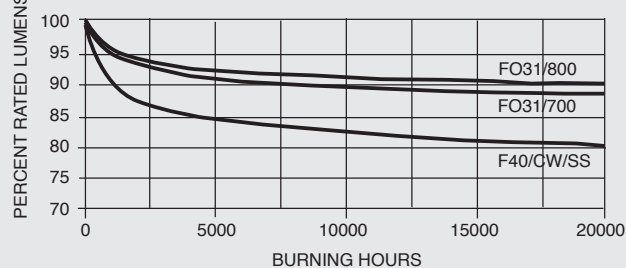
Lamp Lumen Maintenance
